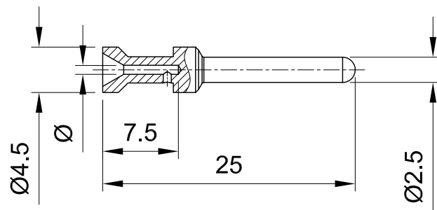
male contact
